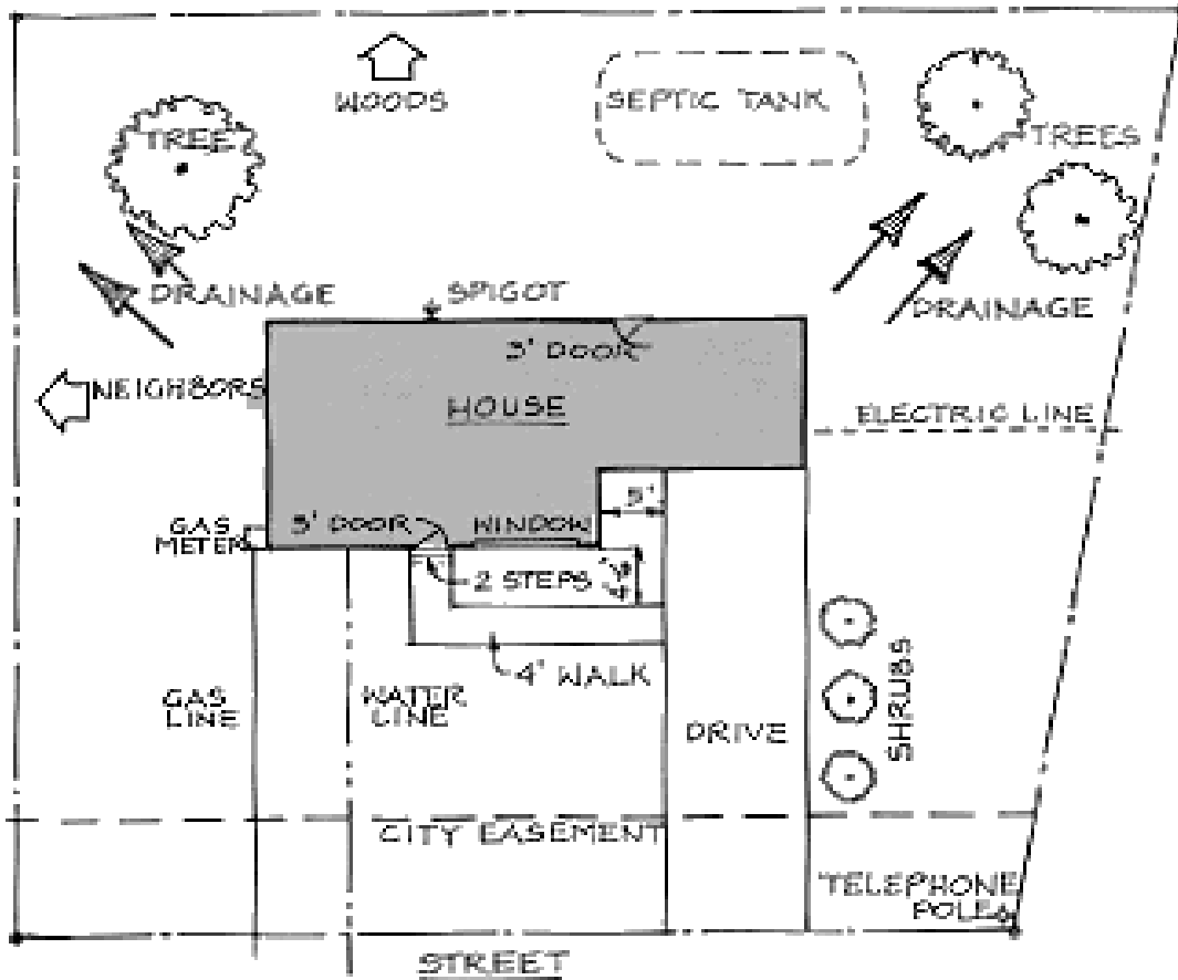
Figure 3. Existing features marked on the plot plan.
